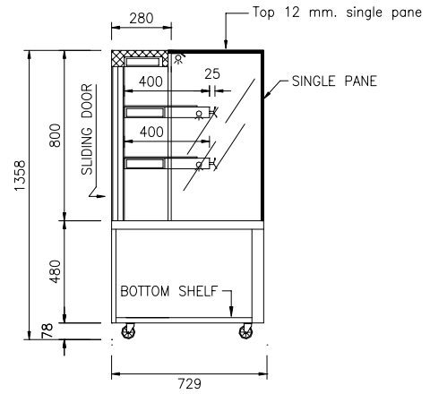
CROSS SECTION
